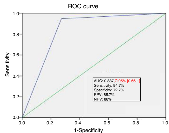
Figure 3 ROC curve showing the ability of PLR induced changes in SV of at least 15% to predict fluid responsiveness. ROC, receiver operating characteristics; PLR, passive leg raising; SV, stroke volume; AUC, area under the curve; PPV, positive predictive value; NPV, negative predictive value.
