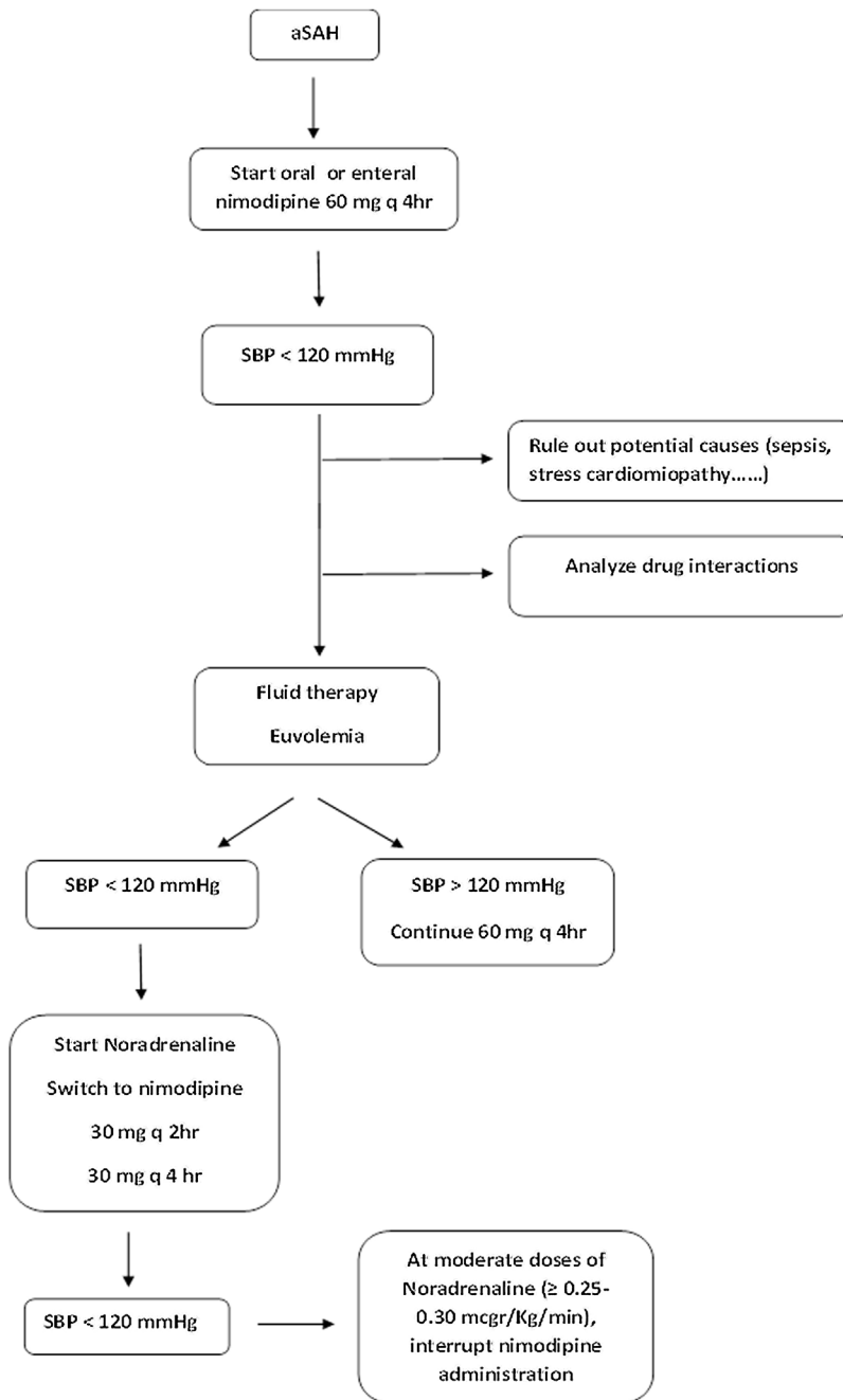
Figure 2 Algorithm management in oral/enteral nimodipine induced hypotension.
